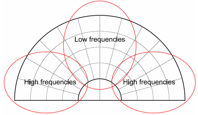
Figure 11. Theatre plan. Scheme with the predominant frequencies of the vessels
